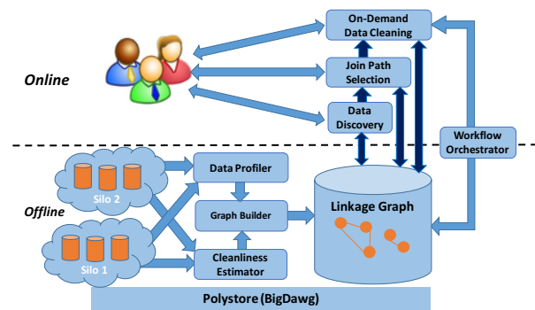
Figure 1: Data Civilizer Architecture
